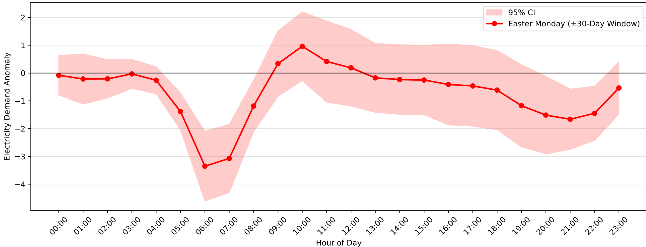
Cronulla Demand Anomaly: Easter Monday (2004–2017, \pm 30 -Day Window)
